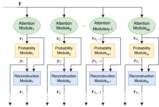
Fig. 11. An illustration of capsule-based attention.
