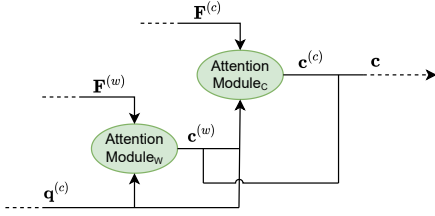
Fig. 7. An illustration of attention-via-attention.
