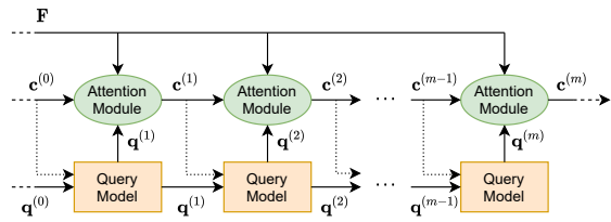
Fig. 10. An example illustration of multi-hop attention. Solid arrows represent the base multi-hop model structure, while dotted arrows represent optional connections.
