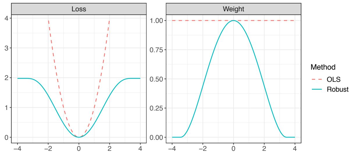
Figure 2. Loss function (left) and assigned weights (right) for OLS regression and the robust MM-regression estimator.
