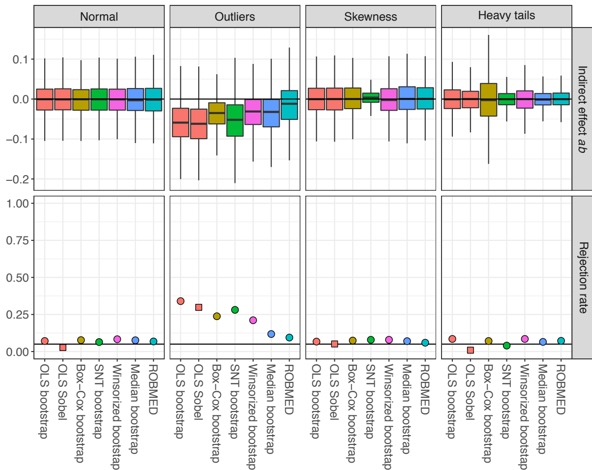
Figure 6. Results from 1000 simulation runs for the simulation setting with no mediation ( a = 0.4, b = 0 ). The top row contains box plots of the estimates of the indirect effect and includes a horizontal reference line for the true indirect effect ab = 0 . Points outside the whiskers are not displayed for better readability. The bottom row displays the rejection rate of the corresponding tests (i.e., the realized size), and a horizontal line is drawn for the nominal size \alpha = 0.05 (the closer to this line the better). The columns correspond to the four investigated settings for error distributions and outliers.
