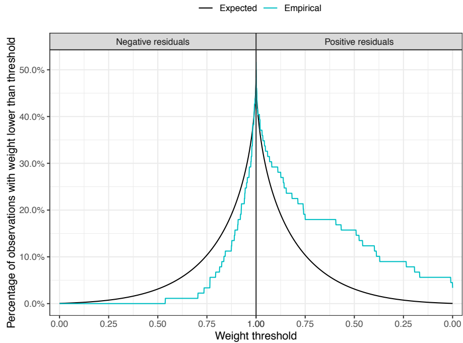
Figure 4. Diagnostic plot of weights from robust regression of task conflict on value diversity. The horizontal axis contains different weight thresholds, and the vertical axis displays the percentage of observations that have a weight below this threshold. A black reference line indicates the expected percentages under normally distributed errors. Observations with negative and positive residuals are shown separately to make it possible to distinguish between symmetric and asymmetric deviations from normality.
