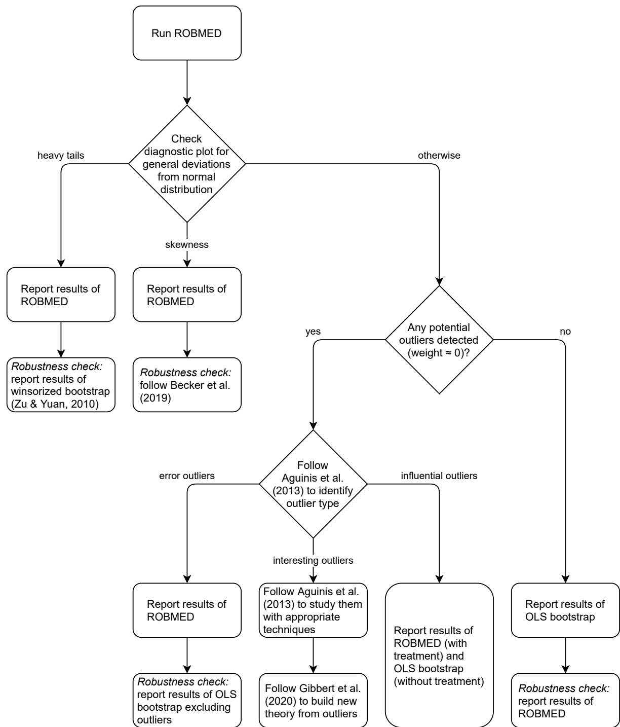
Figure 7. Flowchart of practical guidelines for using ROBMED.
