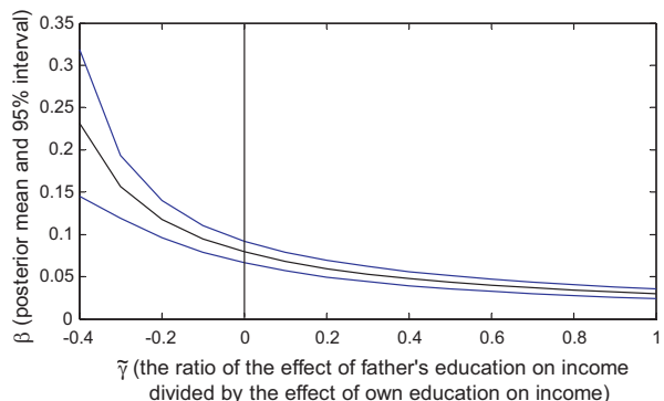
Fig. 2. The mean and the 2.5% and 97.5% percentiles of the posterior distribution of \beta , the effect of (years of) education on the logarithm of income, for different values of \tilde{\gamma} , the ratio of the effect of the father's education on the logarithm of income to the effect of own education on the logarithm of income.
