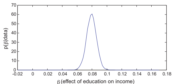
Fig. 1. The posterior density p(\beta|\text{data}) of \beta , the effect of (years of) education on the logarithm of income, when perfect validity of the instrument is assumed.
