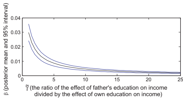
Fig. 3. The mean and the 2.5% and 97.5% percentiles of the posterior distribution of \beta , the effect of (years of) education on the logarithm of income, for different values of \tilde{\gamma} , the ratio of the effect of the father's education on the logarithm of income to the effect of own education on the logarithm of income.
