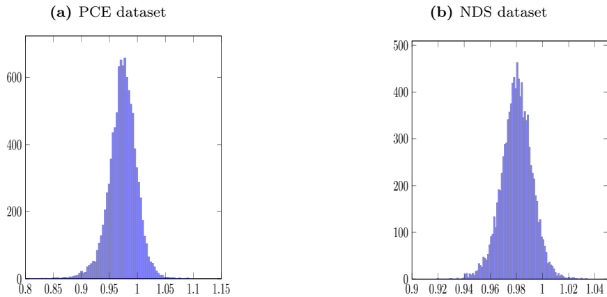
Figure 7: Posterior distribution of the discount factor \rho
