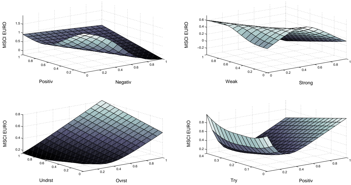
Figure. 6: Fuzzy inference system output surface for selected pairs of inputs (FGFA)
