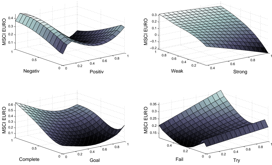
Figure. 5: Fuzzy inference system output surface for selected pairs of inputs (AFA)
