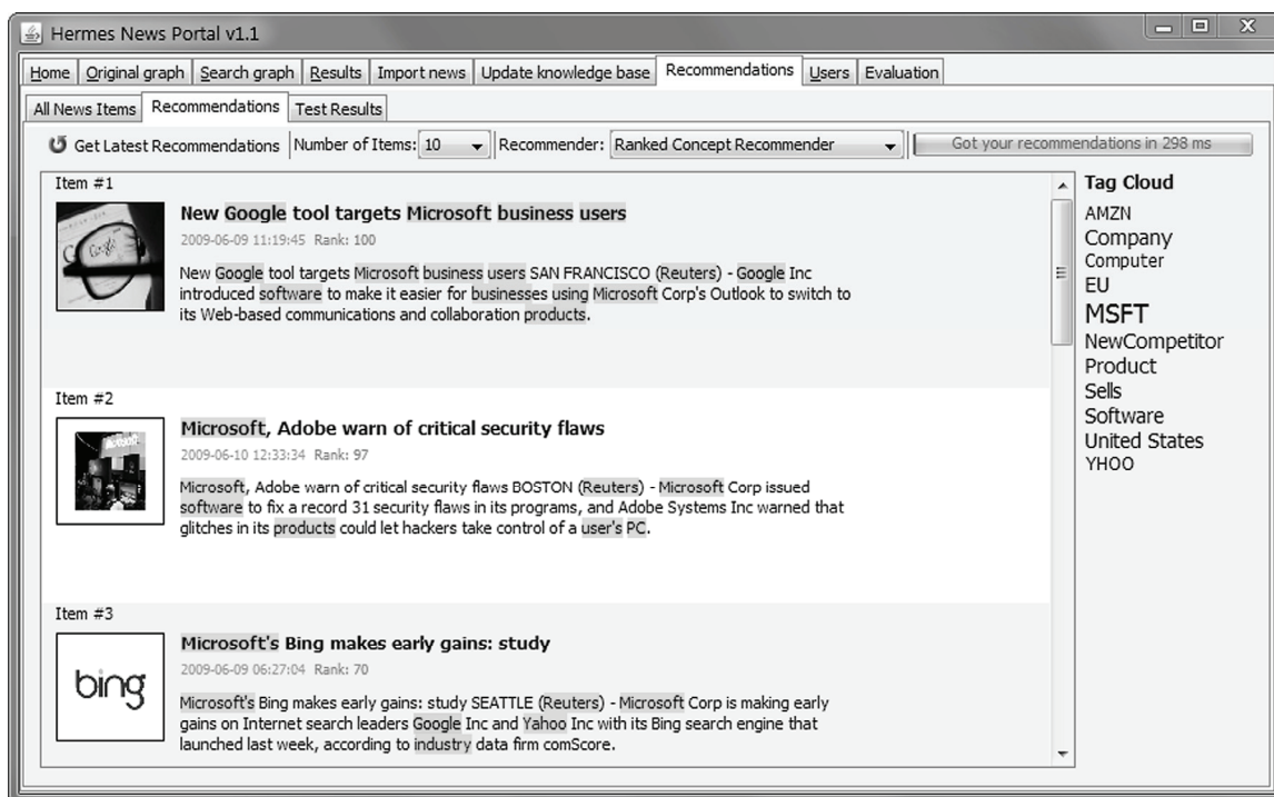
Figure 1. Athena Recommendations
