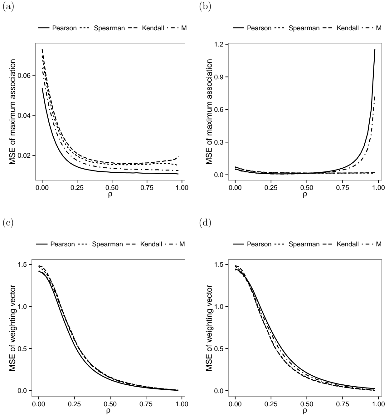
Figure 3: MSEs of the maximum association measures ( top ) and the weighting vectors ( bottom ) for the correctly specified model ( left ) and for the misspecified model ( right ). In (b) and (d), the lines for the Spearman and Kendall correlation almost coincide. In (c), the lines for all methods except the Pearson correlation almost coincide.
